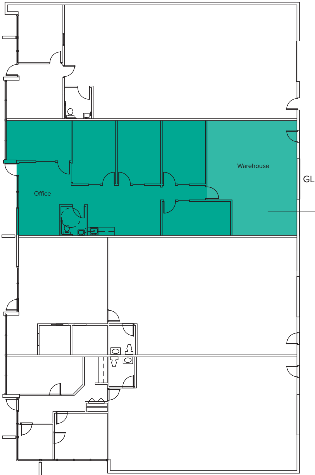
1 MAIN FLOOR PLAN - BUILDING "D" NOT TO SCALE
